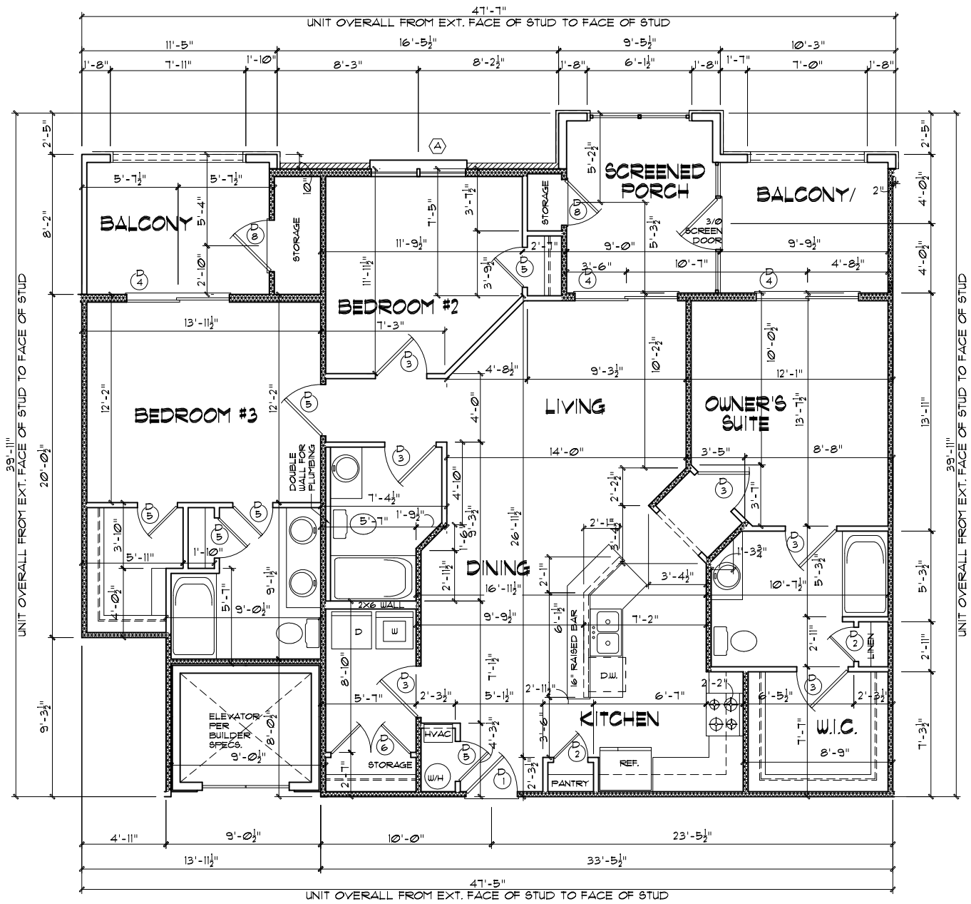
FIRST FLOOR UNIT PLAN UNIT TYPE U0058 SCALE: 1/4" = 1'-0" REAR UNIT
