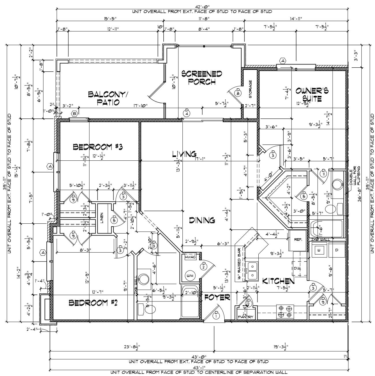
FIRST FLOOR UNIT PLAN UNIT TYPE U0056 SCALE: 1/4" = 1'-0"
